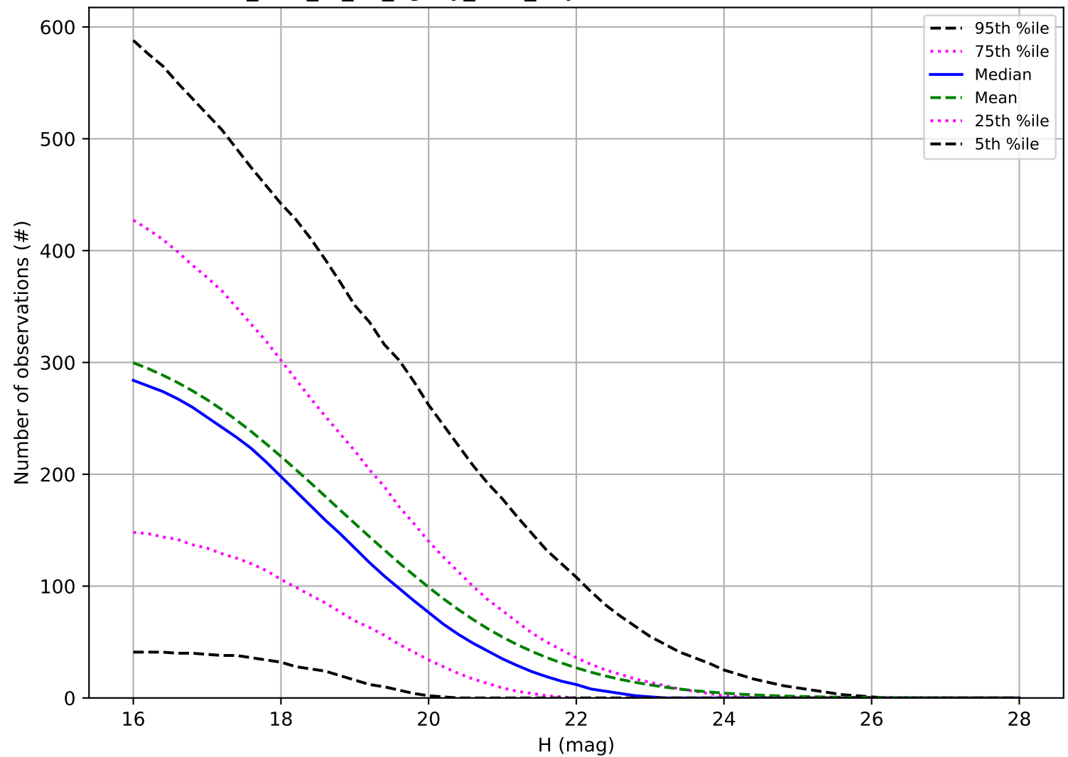
too_elab_r8_d2_ugrizy_v3.4_10yrs: Number of observations PHA
