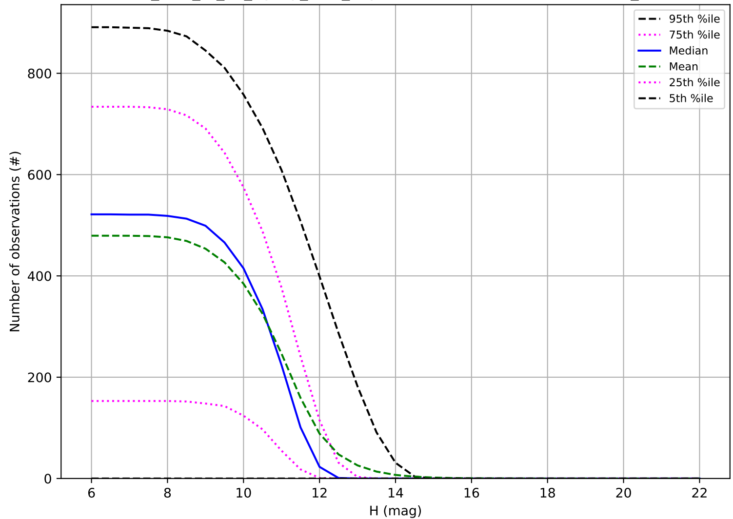
too_elab_r8_d2_ugrizy_v3.4_10yrs: Number of observations OCC_r20
