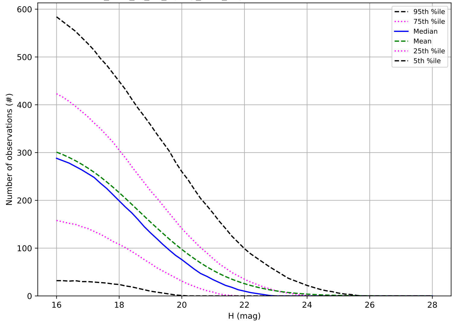
too_elab_r8_d2_ugrizy_v3.4_10yrs: Number of observations NEO
