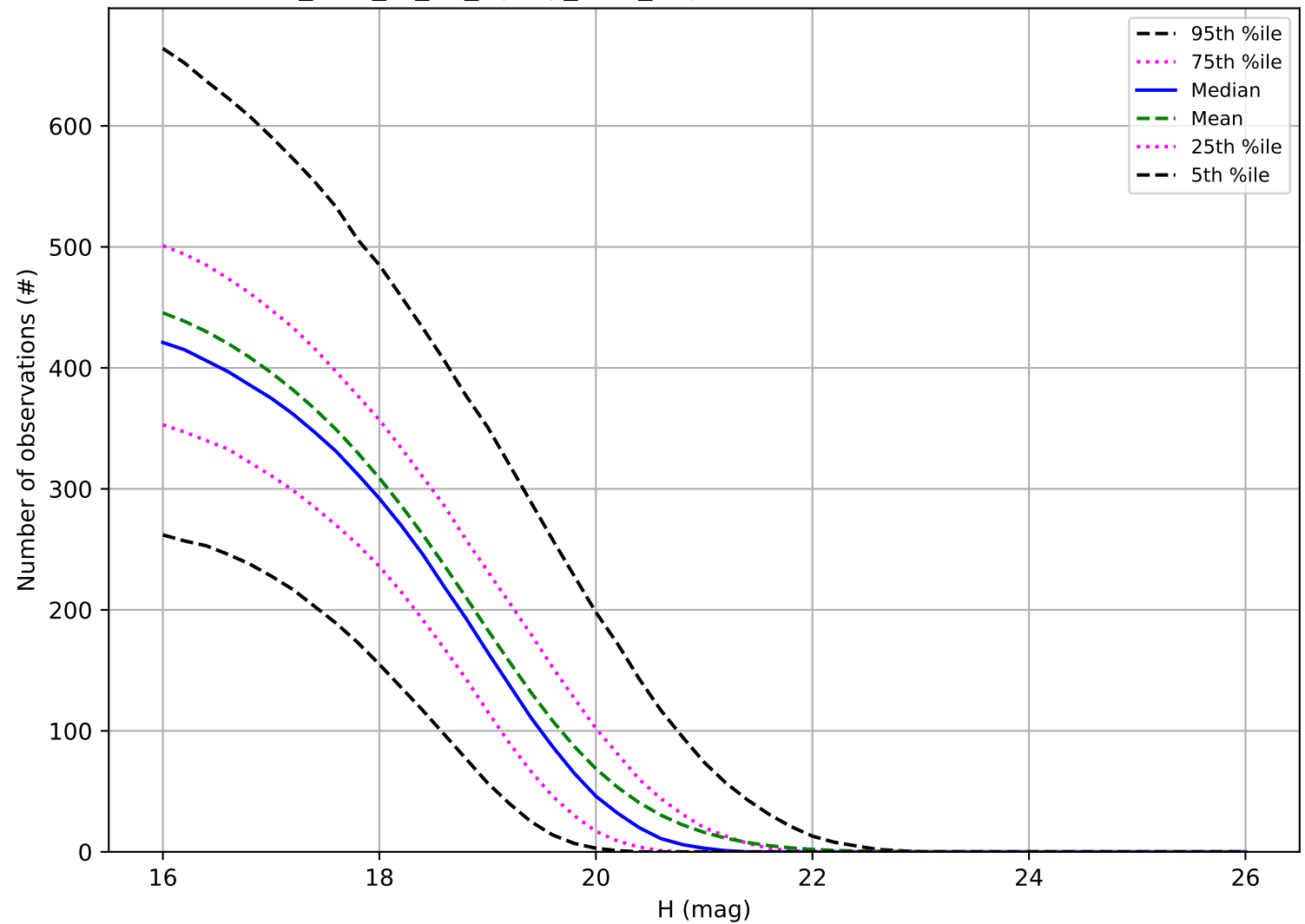
too_elab_r8_d2_ugrizy_v3.4_10yrs: Number of observations MBA
