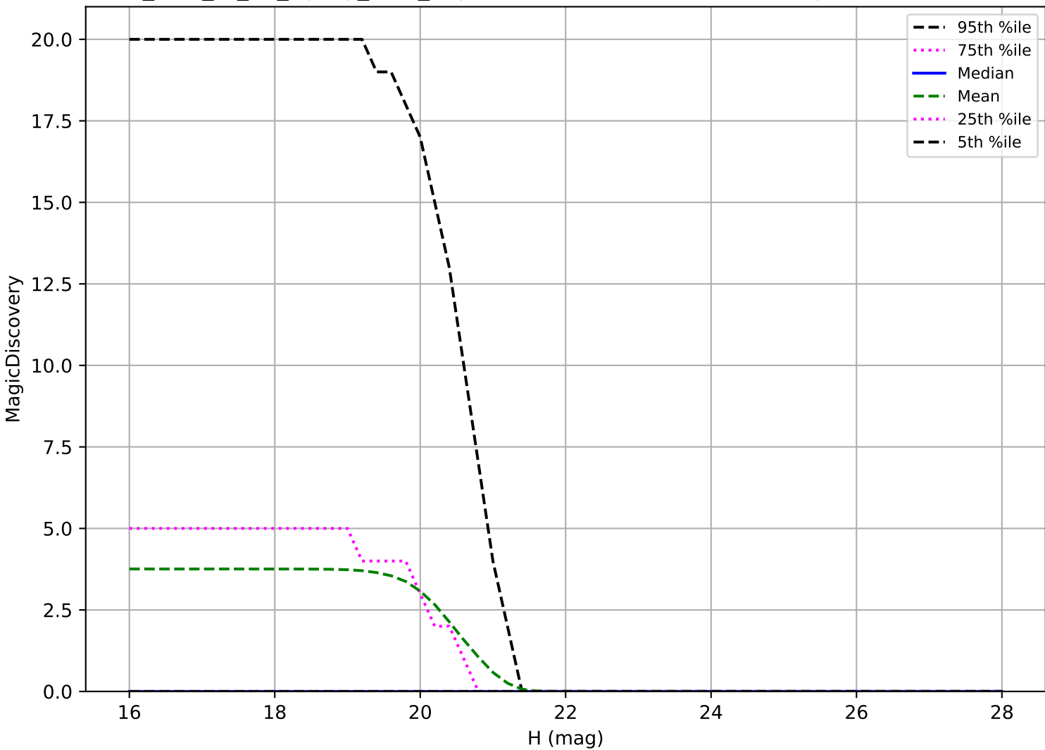
too_elab_r8_d2_ugrizy_v3.4_10yrs: Vatira 6 detections in 60 nights detection loss
