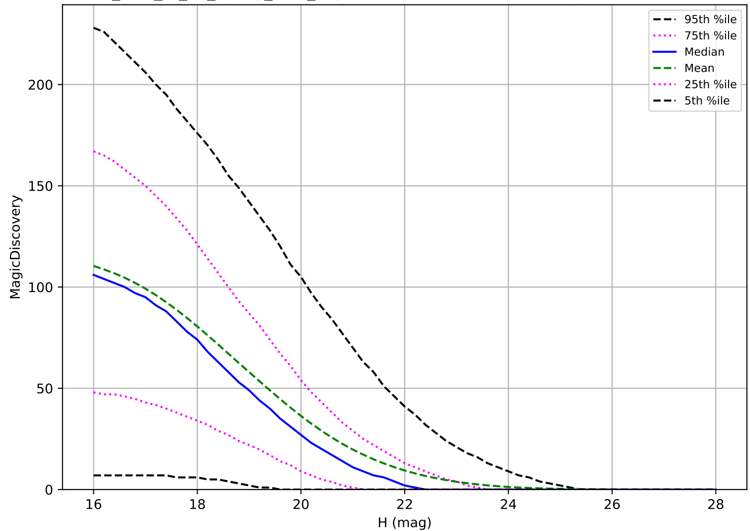
too_elab_r8_d2_ugrizy_v3.4_10yrs: PHA 6 detections in 60 nights detection loss
