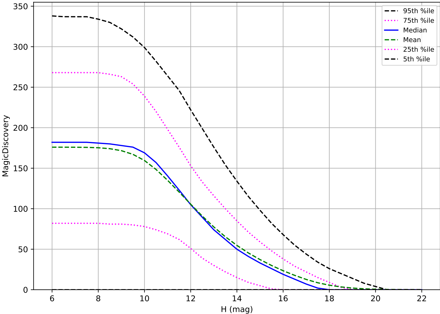
too_elab_r8_d2_ugrizy_v3.4_10yrs: OCC_r5 6 detections in 60 nights detection loss
