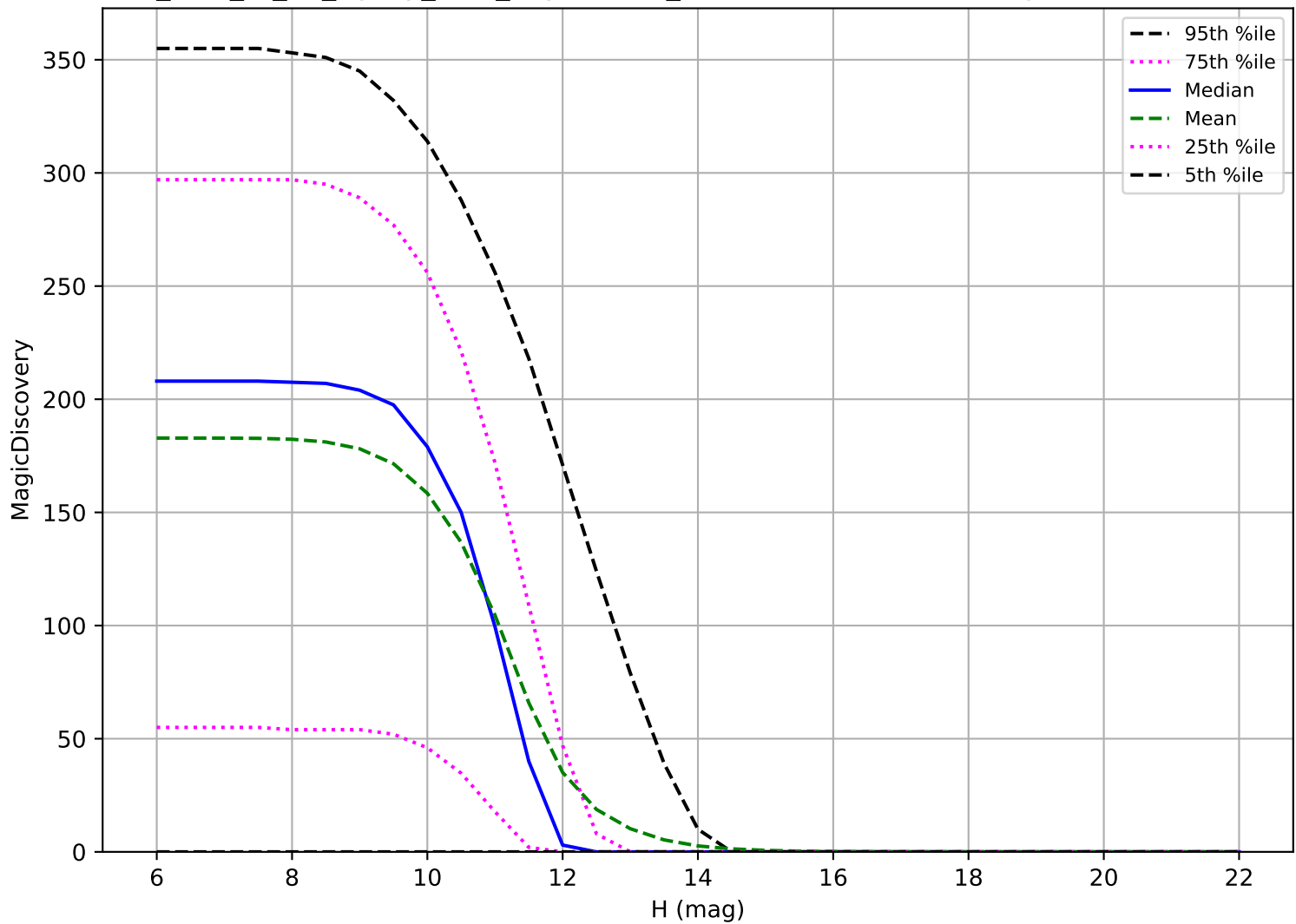
too_elab_r8_d2_ugrizy_v3.4_10yrs: OCC_r20 6 detections in 60 nights detection loss
