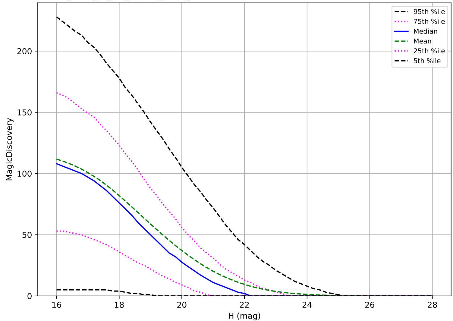
too_elab_r8_d2_ugrizy_v3.4_10yrs: NEO 6 detections in 60 nights detection loss
