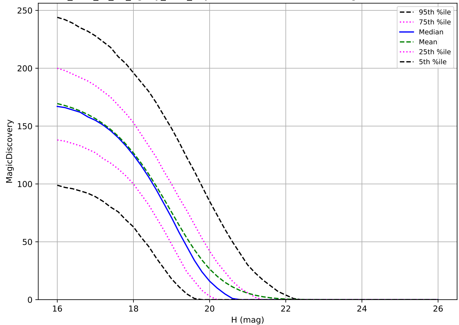
too_elab_r8_d2_ugrizy_v3.4_10yrs: MBA 6 detections in 60 nights detection loss
