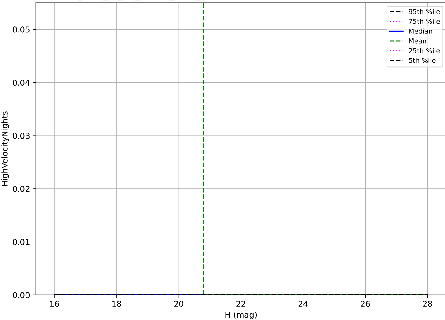
too_elab_r8_d2_ugrizy_v3.4_10yrs: Vatira High velocity pair detection loss
