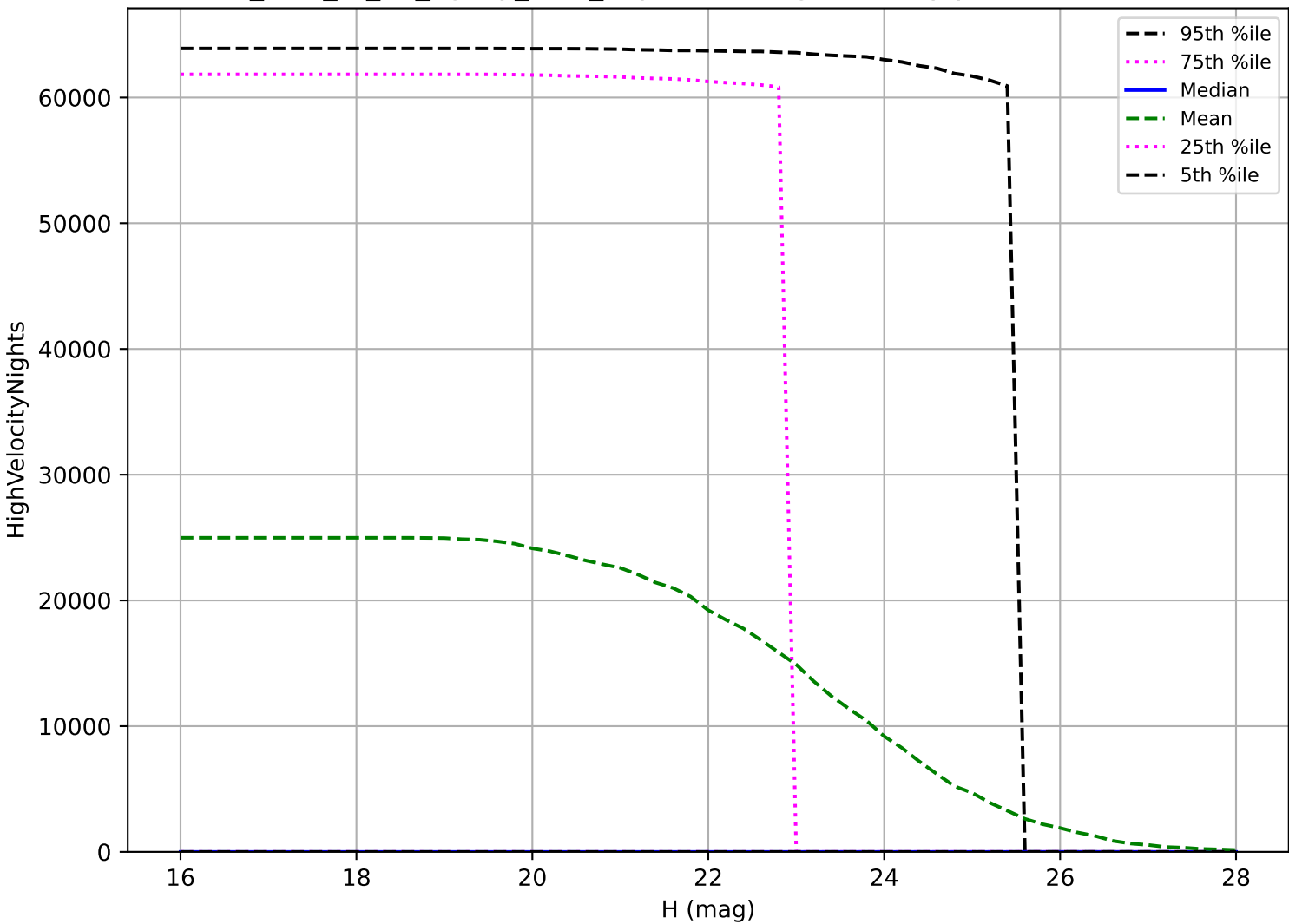
too_elab_r8_d2_ugrizy_v3.4_10yrs: PHA High velocity pair detection loss
