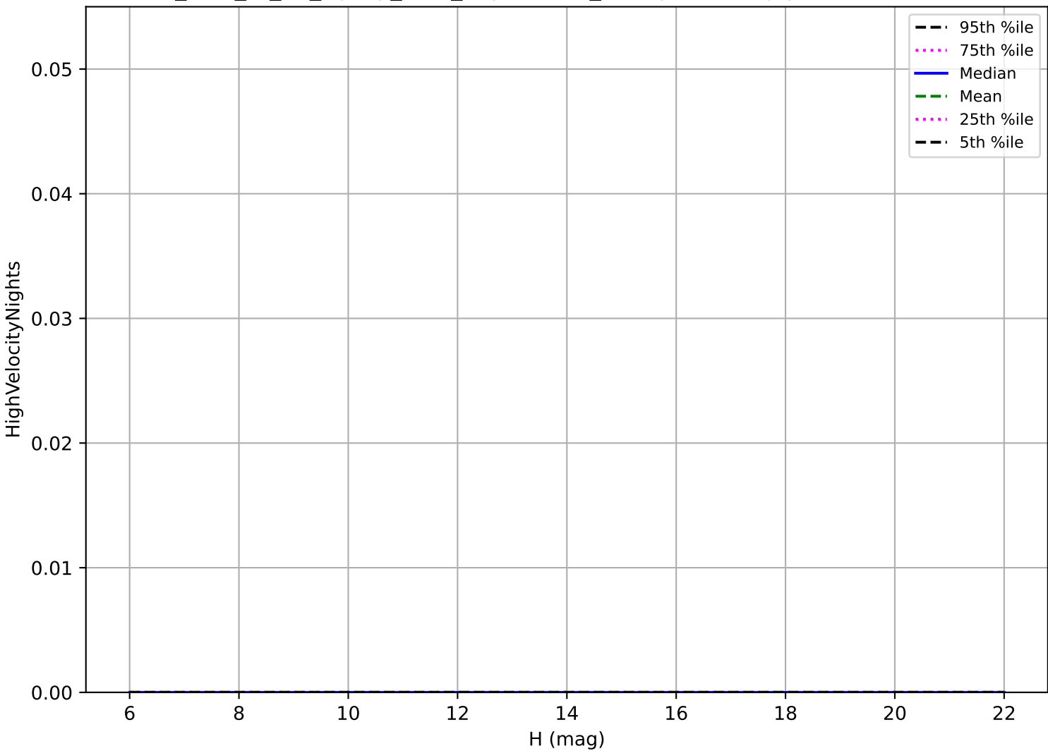
too_elab_r8_d2_ugrizy_v3.4_10yrs: OCC_r5 High velocity pair detection loss
