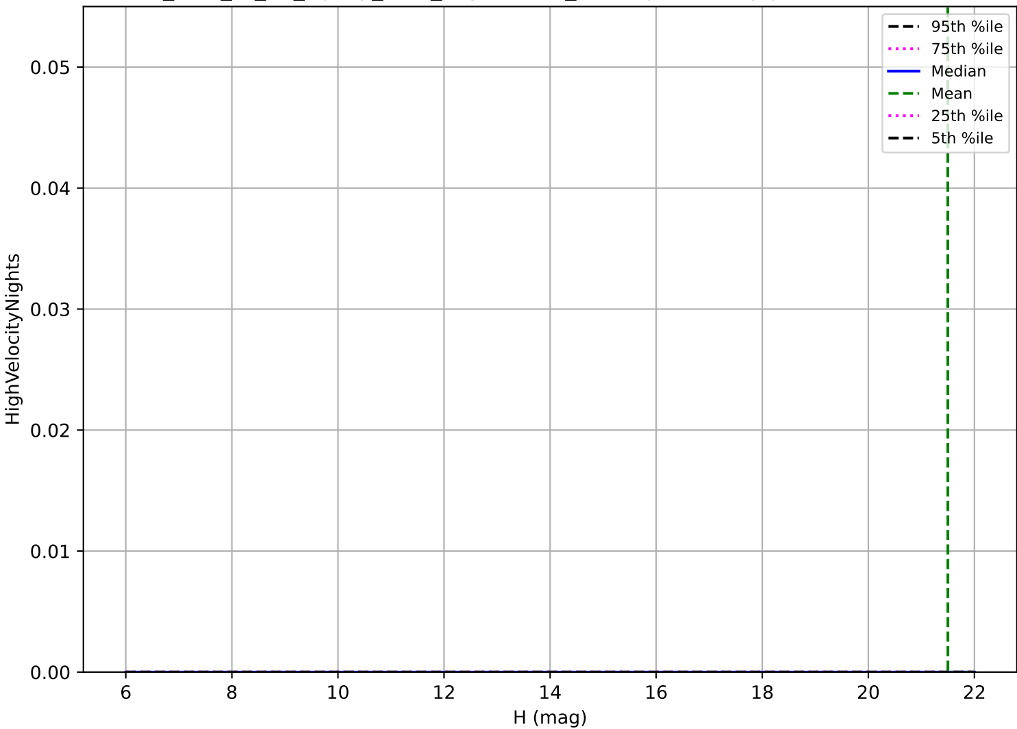
too_elab_r8_d2_ugrizy_v3.4_10yrs: OCC_r20 High velocity pair detection loss
