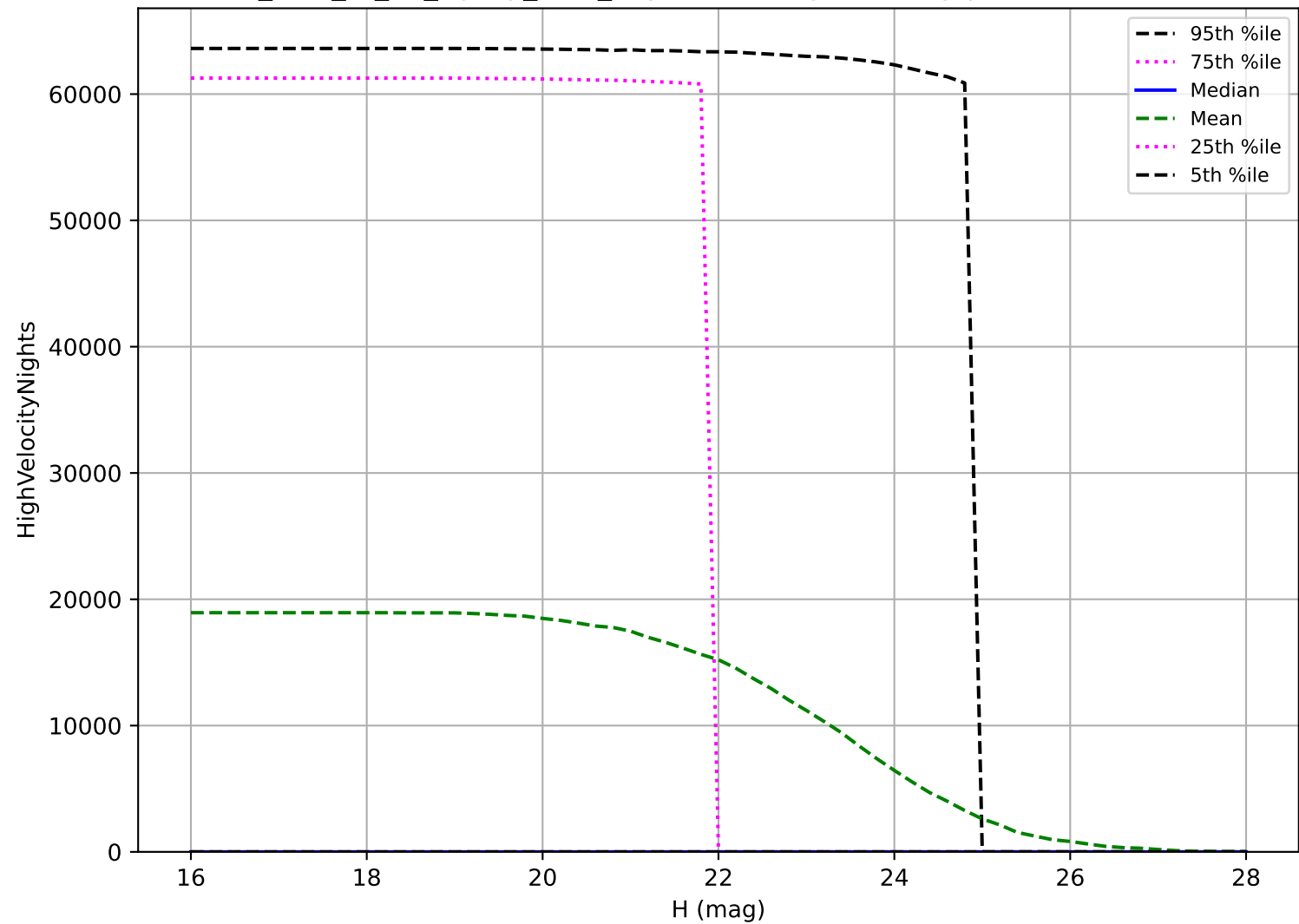
too_elab_r8_d2_ugrizy_v3.4_10yrs: NEO High velocity pair detection loss
