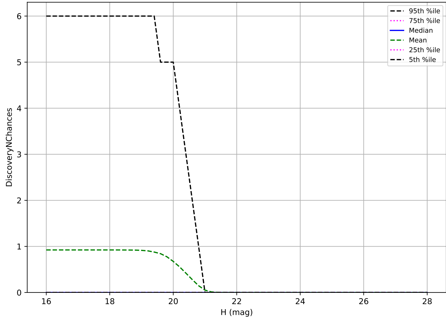
too_elab_r8_d2_ugrizy_v3.4_10yrs: Vatira 3 pairs in 15 nights detection loss
