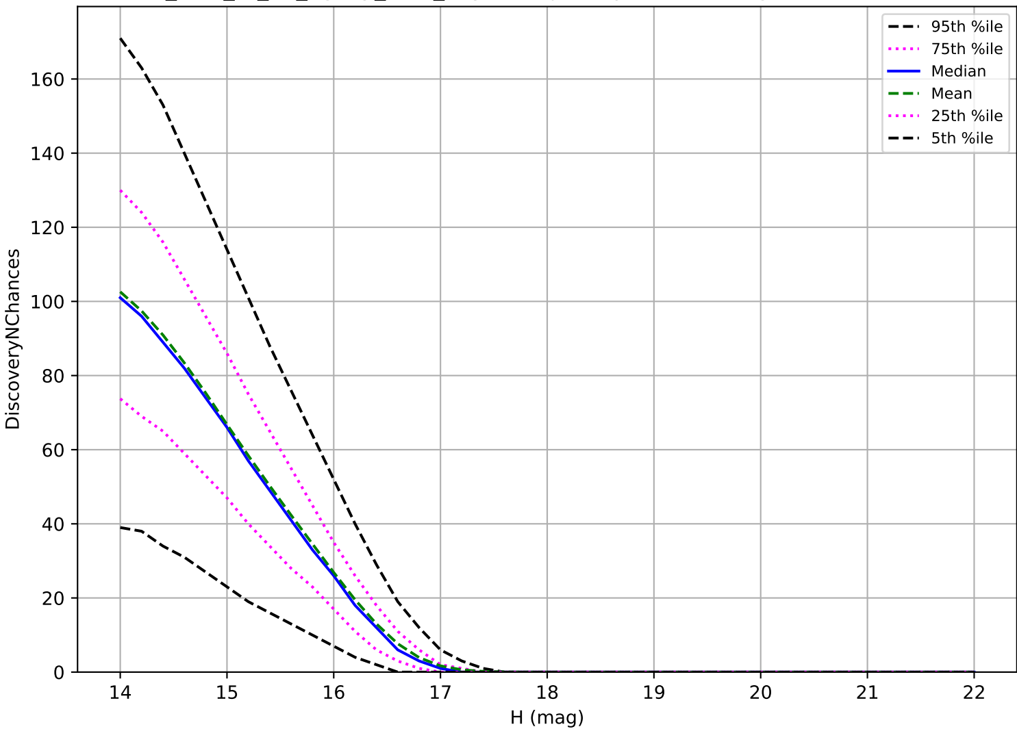
too_elab_r8_d2_ugrizy_v3.4_10yrs: Trojan 3 pairs in 15 nights detection loss
