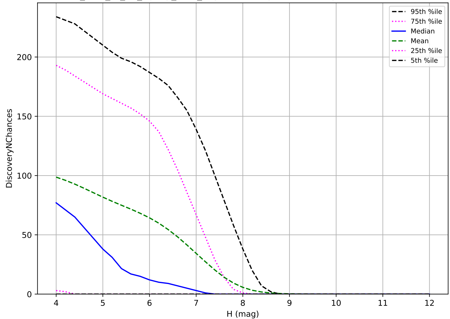
too_elab_r8_d2_ugrizy_v3.4_10yrs: TNO 3 pairs in 15 nights detection loss
