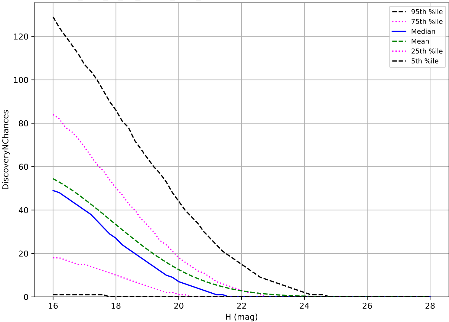
too_elab_r8_d2_ugrizy_v3.4_10yrs: PHA 3 pairs in 15 nights detection loss
