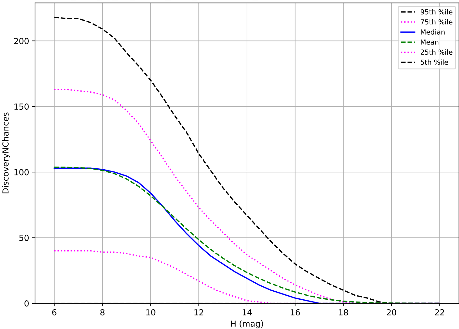
too_elab_r8_d2_ugrizy_v3.4_10yrs: OCC_r5 3 pairs in 15 nights detection loss
