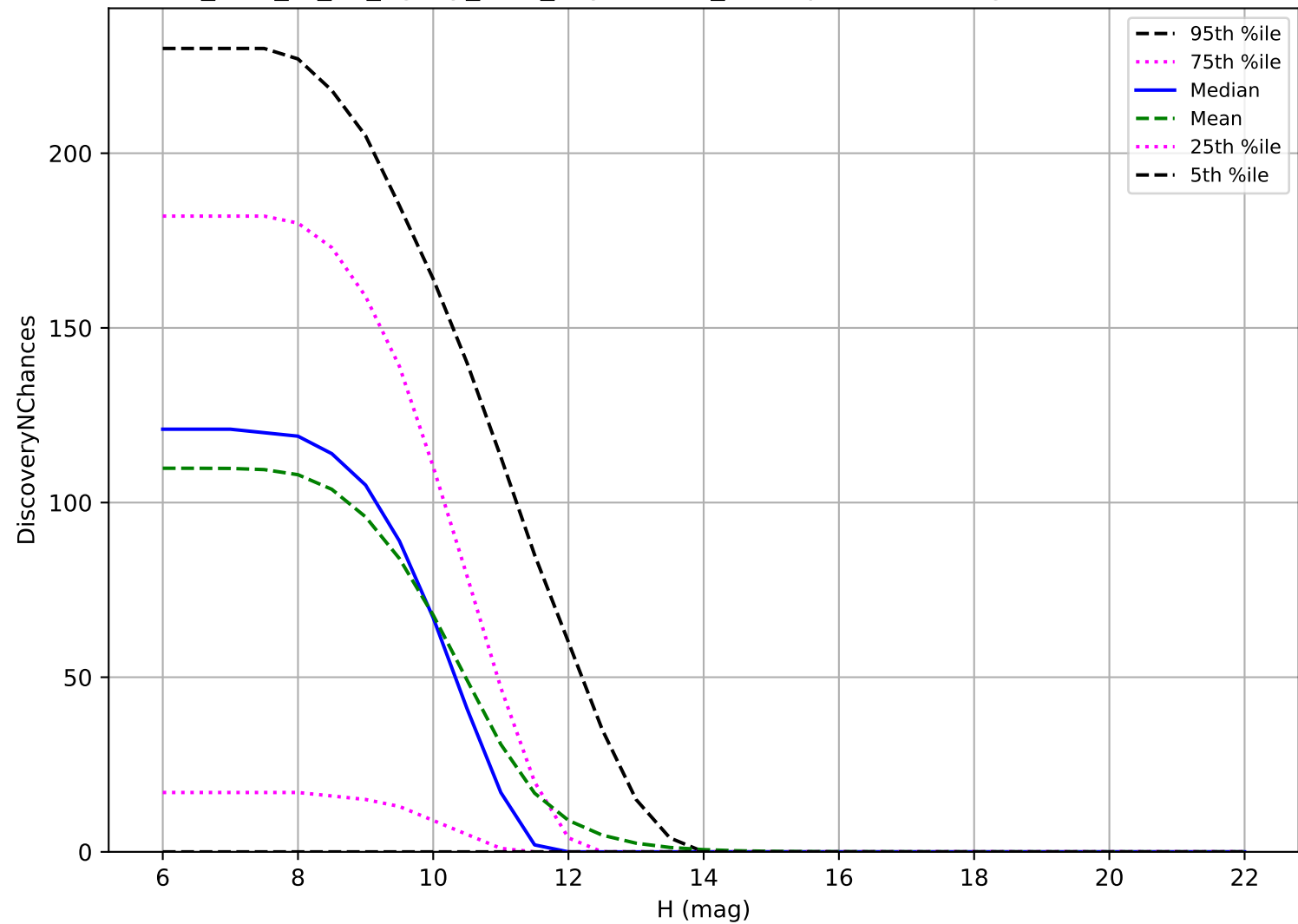
too_elab_r8_d2_ugrizy_v3.4_10yrs: OCC_r20 3 pairs in 15 nights detection loss
