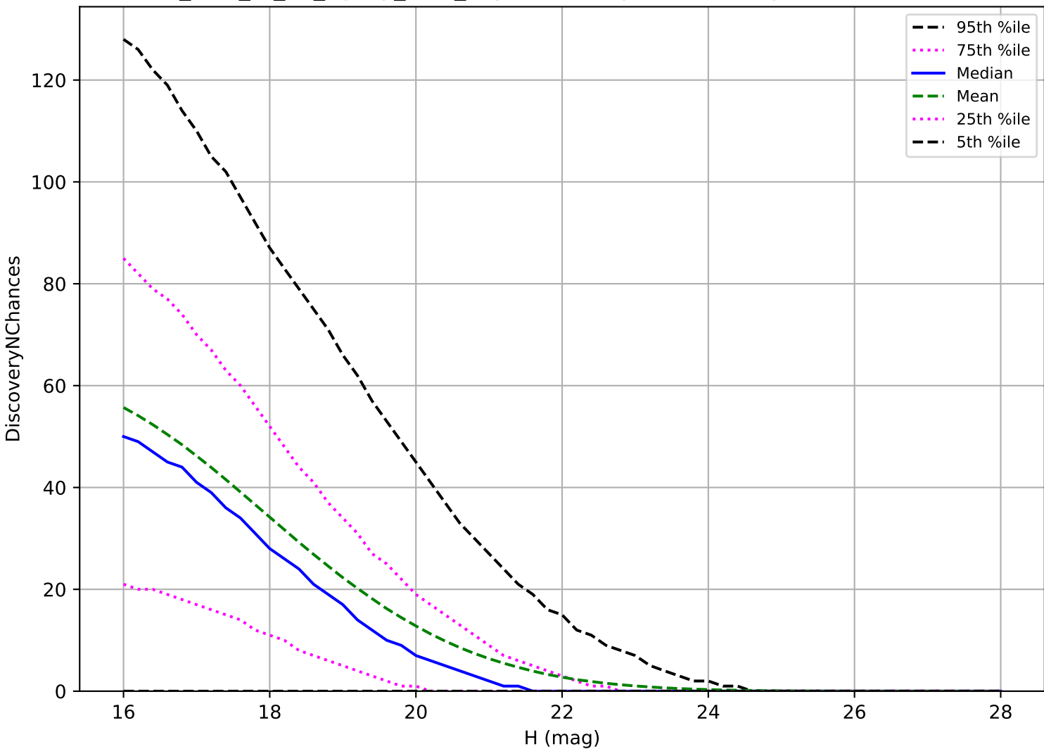
too_elab_r8_d2_ugrizy_v3.4_10yrs: NEO 3 pairs in 15 nights detection loss
