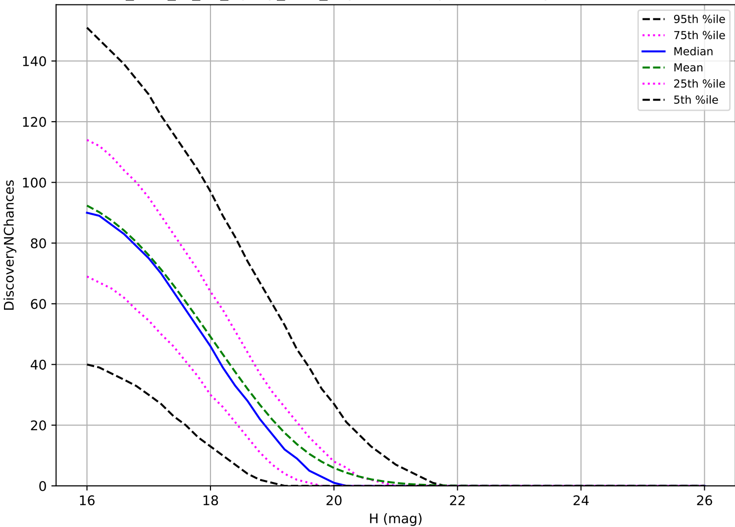
too_elab_r8_d2_ugrizy_v3.4_10yrs: MBA 3 pairs in 15 nights detection loss
