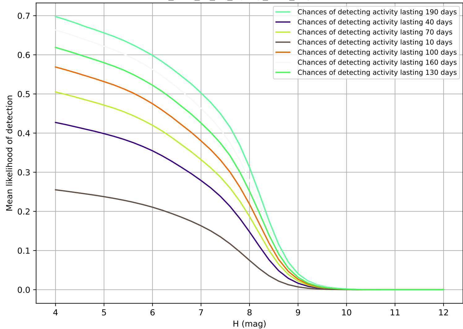
too_elab_r8_d2_ugrizy_v3.4_10yrs TNO
