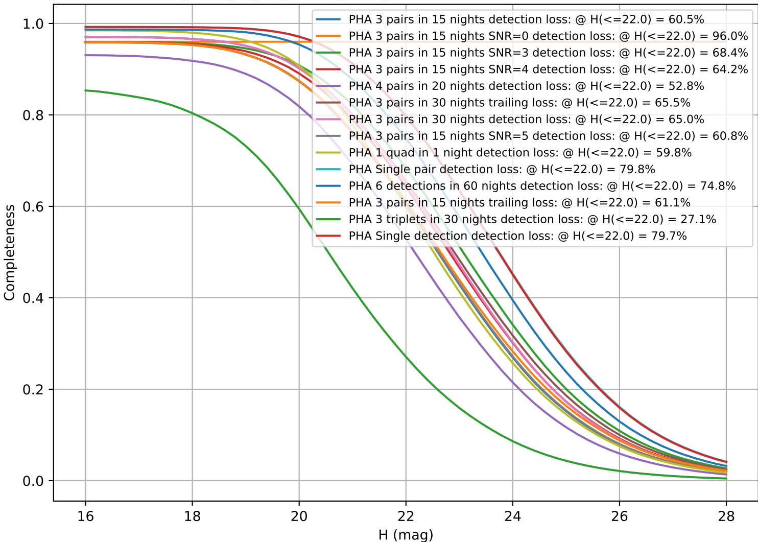
too_elab_r8_d2_ugrizy_v3.4_10yrs: CumulativeCompleteness
