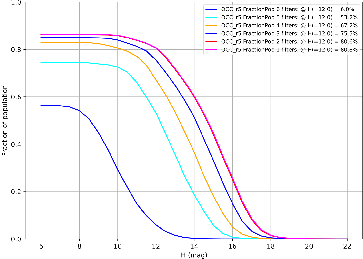
too_elab_r8_d2_ugrizy_v3.4_10yrs: Fraction of population with colors in X filters OCC_r5
