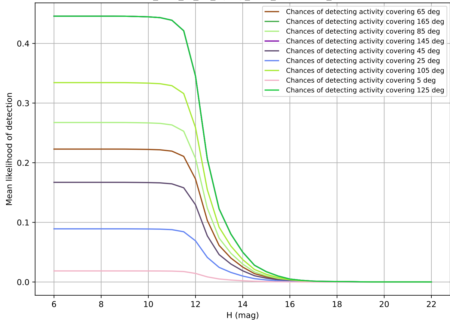
too_elab_r8_d2_ugrizy_v3.4_10yrs OCC_r20
