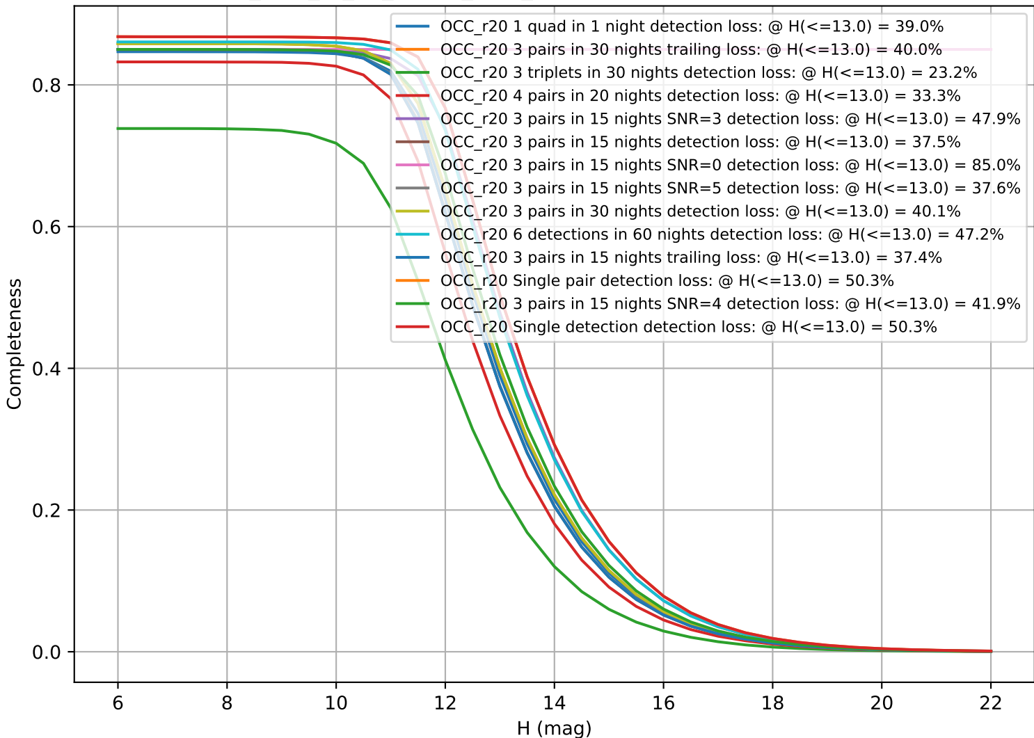
too_elab_r8_d2_ugrizy_v3.4_10yrs: CumulativeCompleteness
