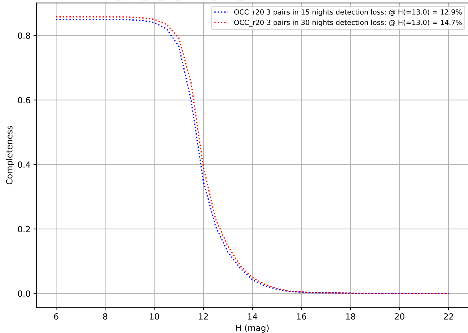
too_elab_r8_d2_ugrizy_v3.4_10yrs: DifferentialCompleteness
