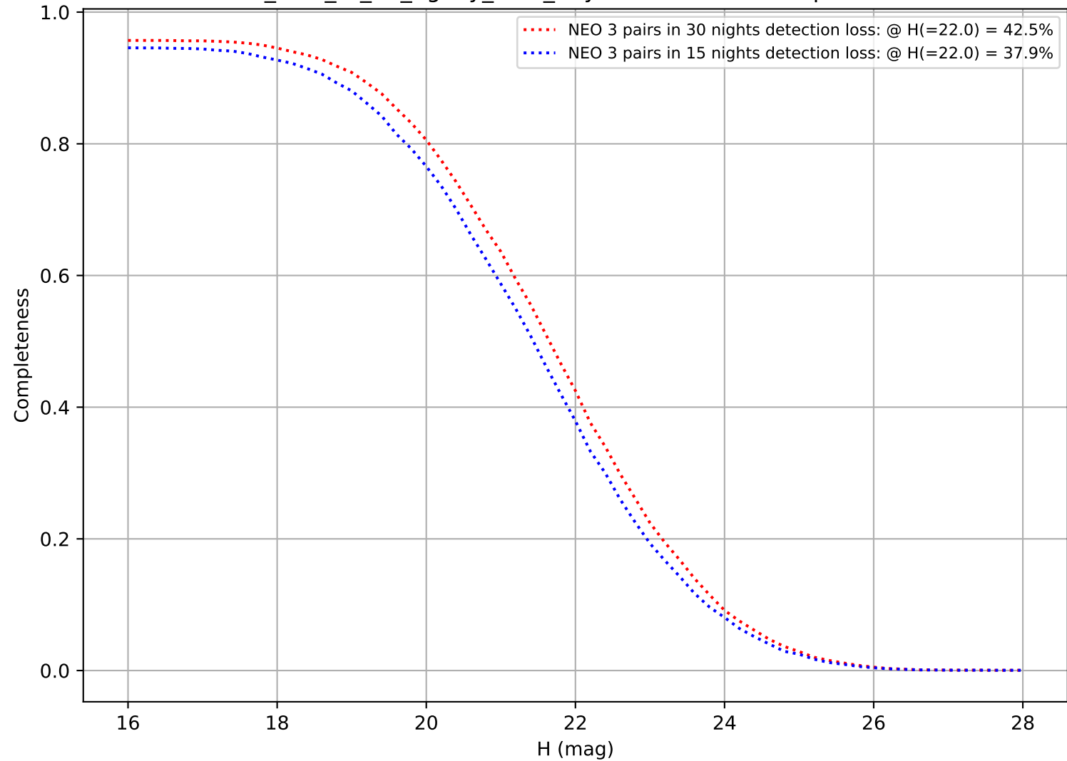
too_elab_r8_d2_ugrizy_v3.4_10yrs: DifferentialCompleteness
