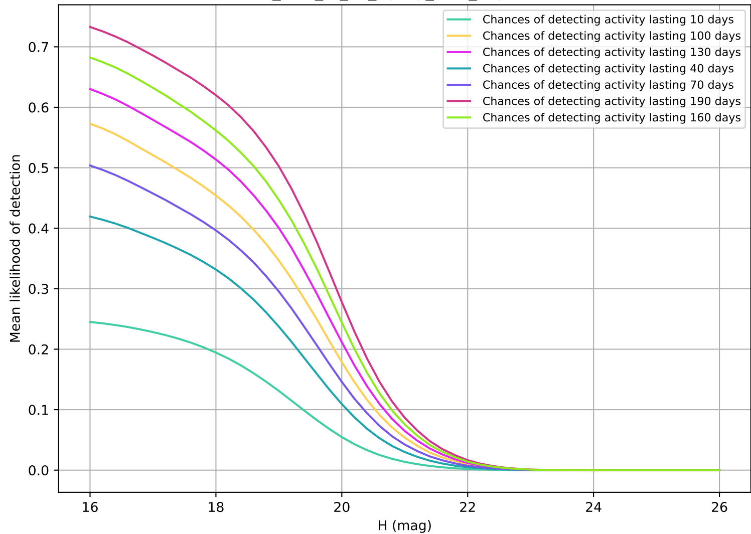
too_elab_r8_d2_ugrizy_v3.4_10yrs MBA
