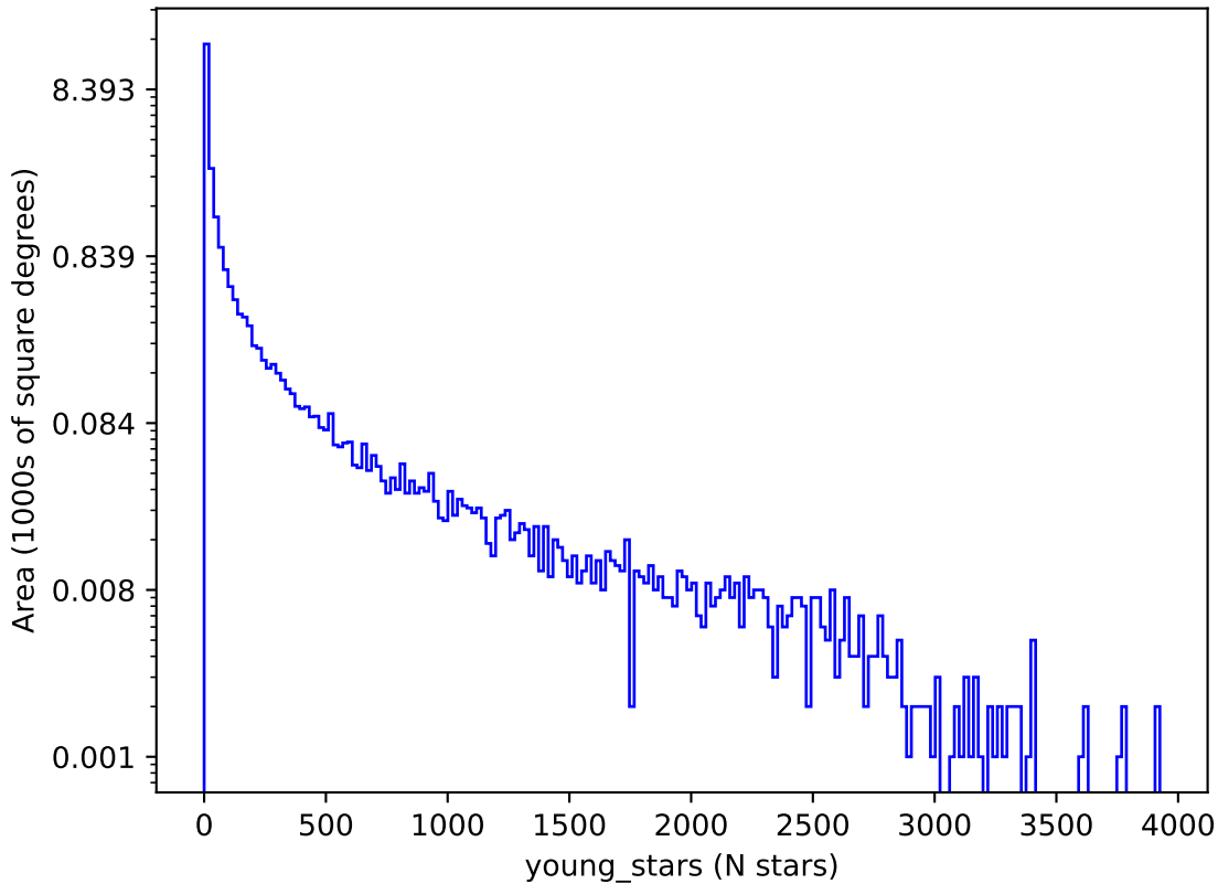
too_elab_r8_d2_ugrizy_v3.4_10yrs : young_stars
