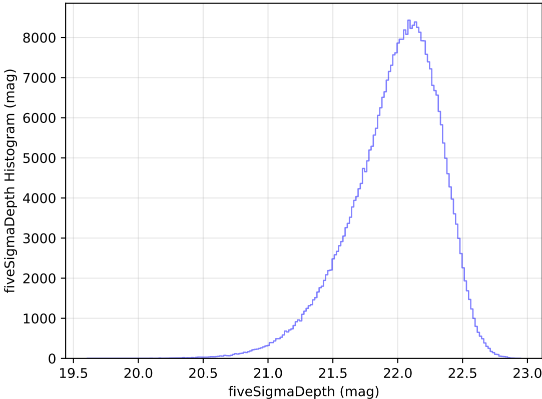
too_elab_r8_d2_ugrizy_v3.4_10yrs y: fiveSigmaDepth Histogram
