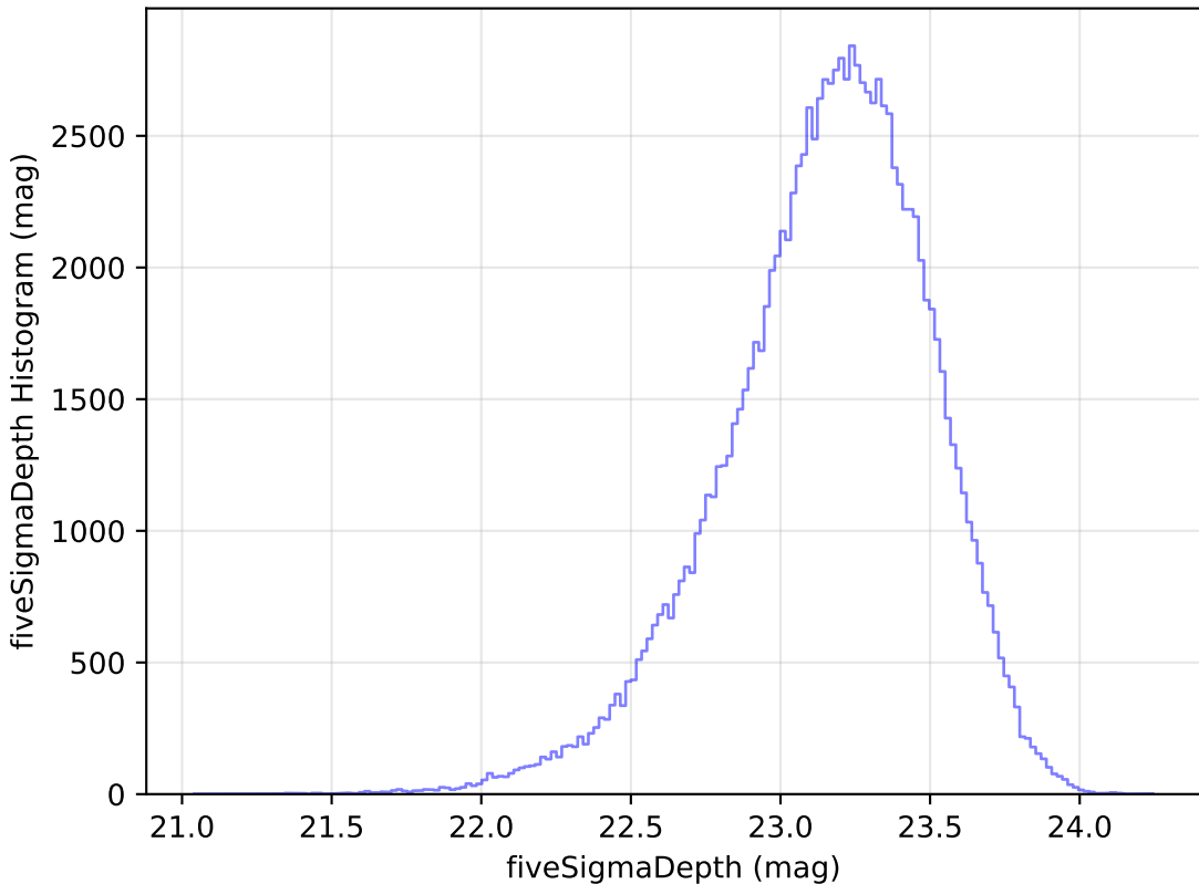
too_elab_r8_d2_ugrizy_v3.4_10yrs u: fiveSigmaDepth Histogram
