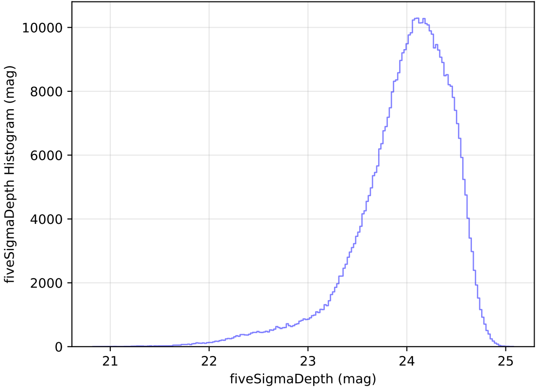
too_elab_r8_d2_ugrizy_v3.4_10yrs r: fiveSigmaDepth Histogram
