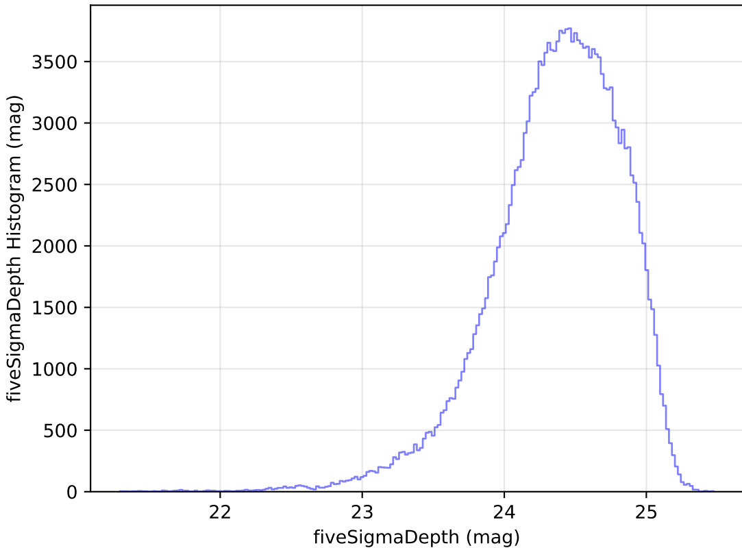
too_elab_r8_d2_ugrizy_v3.4_10yrs g: fiveSigmaDepth Histogram
