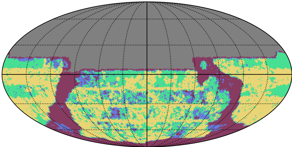
too_elab_r8_d2_ugrizy_v3.4_10yrs u band: YearCoverage night
