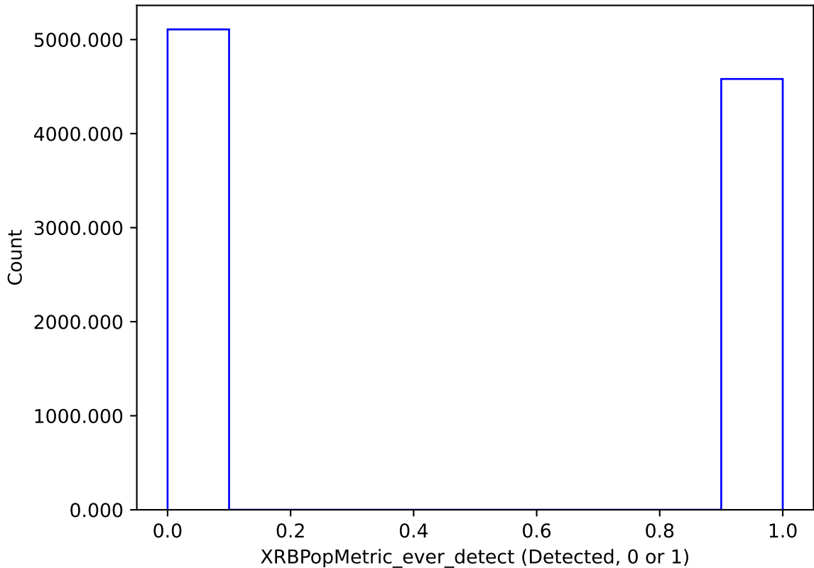
too_elab_r8_d2_ugrizy_v3.4_10yrs : XRBPoMetric_ever_detect
