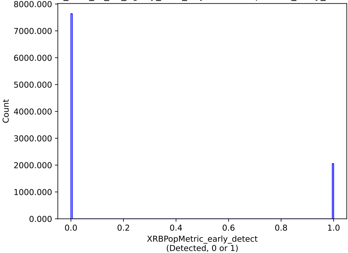
too_elab_r8_d2_ugrizy_v3.4_10yrs : XRBPopMetric_early_detect
