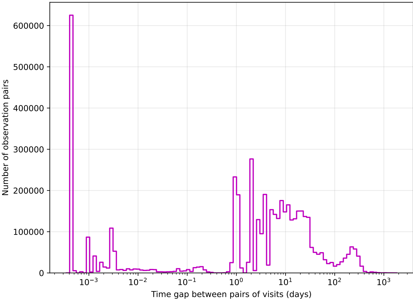
too_elab_r8_d2_ugrizy_v3.4_10yrs z band: Tgaps observationStartMJD
