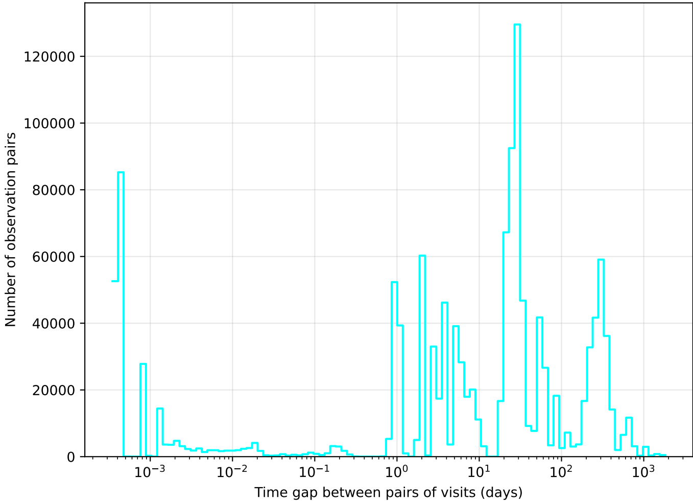
too_elab_r8_d2_ugrizy_v3.4_10yrs u band: Tgaps observationStartMJD
