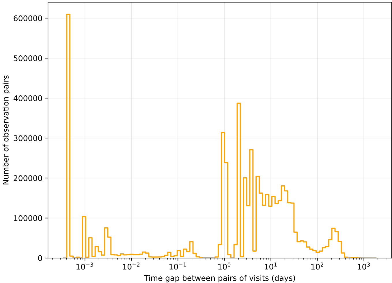
too_elab_r8_d2_ugrizy_v3.4_10yrs r band: Tgaps observationStartMJD
