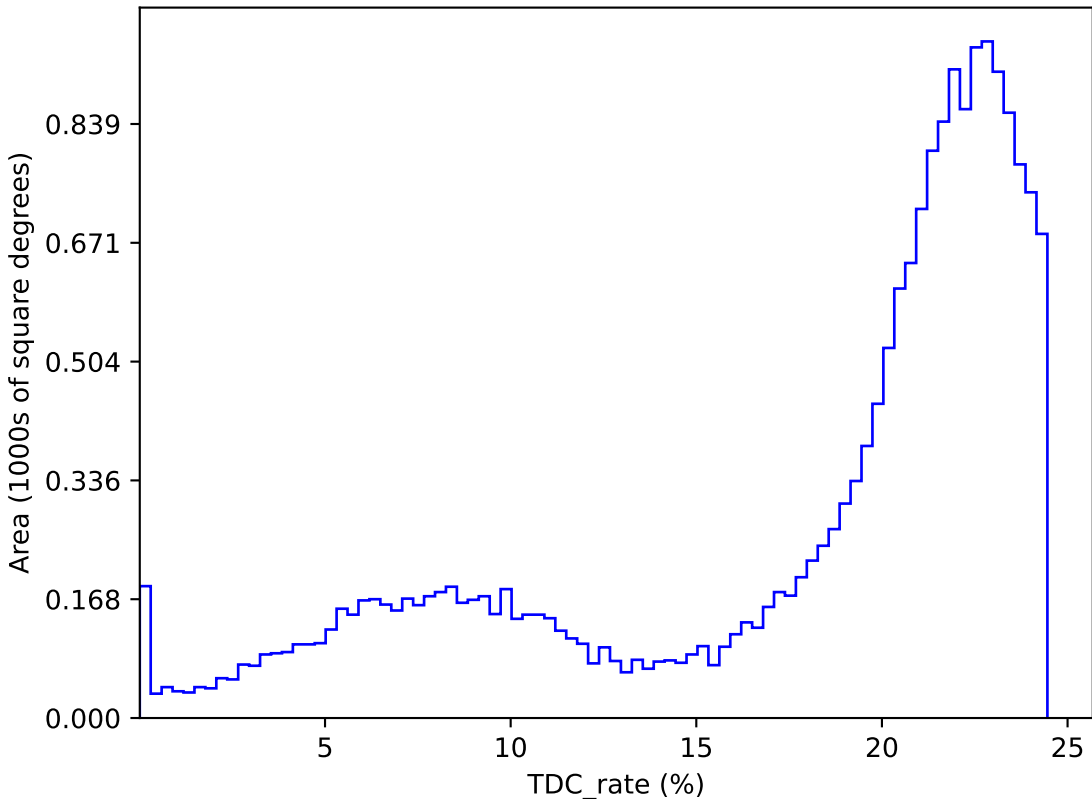
too_elab_r8_d2_ugrizy_v3.4_10yrs : TDC_rate
