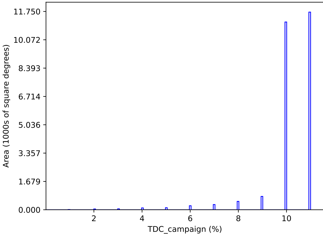
too_elab_r8_d2_ugrizy_v3.4_10yrs : TDC_campaign
