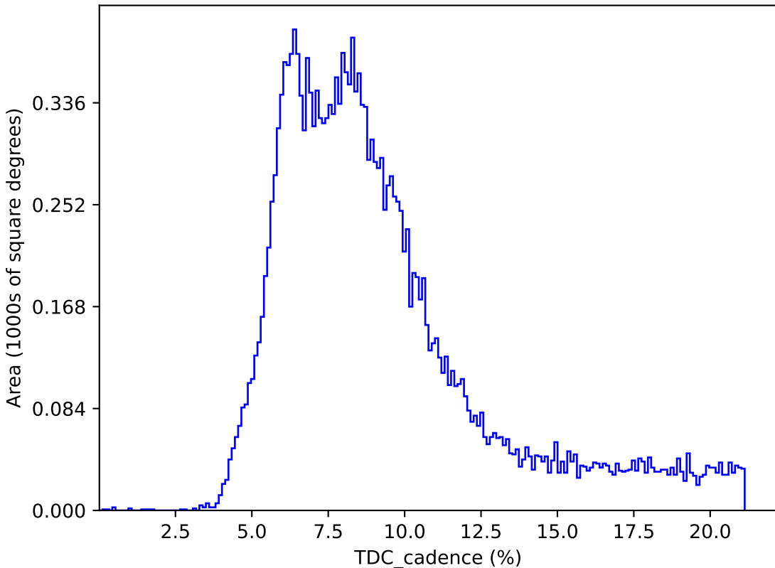
too_elab_r8_d2_ugrizy_v3.4_10yrs : TDC_cadence
