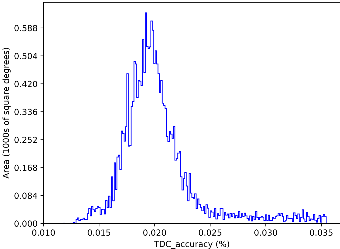
too_elab_r8_d2_ugrizy_v3.4_10yrs : TDC_accuracy
