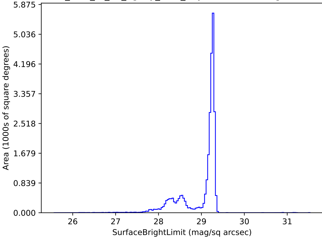
too_elab_r8_d2_ugrizy_v3.4_10yrs z: SurfaceBrightLimit
