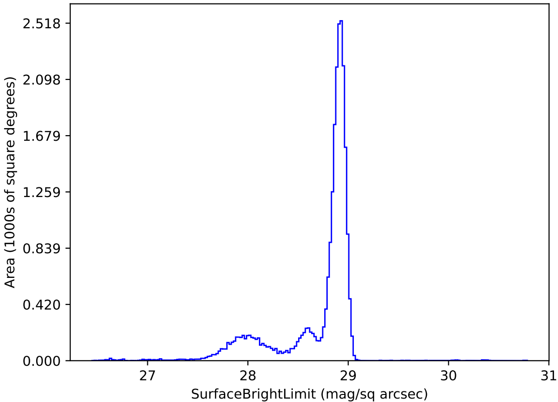
too_elab_r8_d2_ugrizy_v3.4_10yrs u: SurfaceBrightLimit
