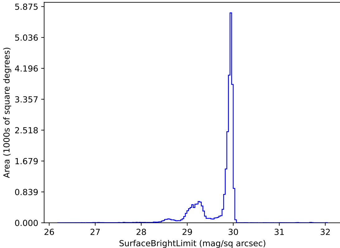
too_elab_r8_d2_ugrizy_v3.4_10yrs i: SurfaceBrightLimit
