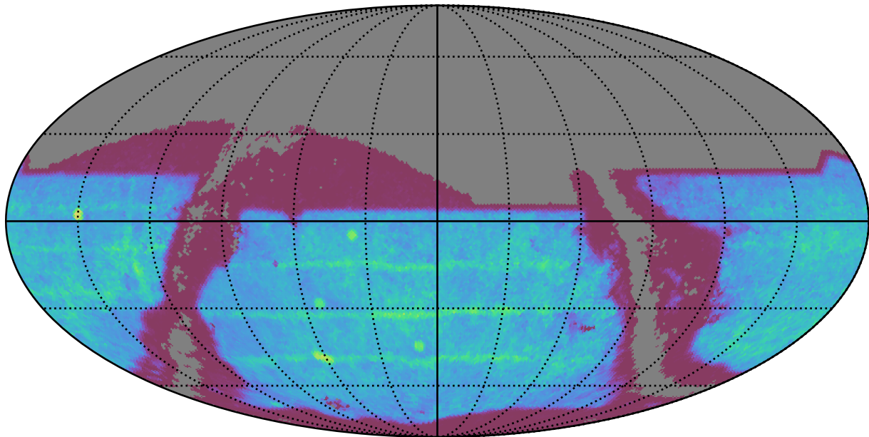
too_elab_r8_d2_ugrizy_v3.4_10yrs : SNSLMetric
